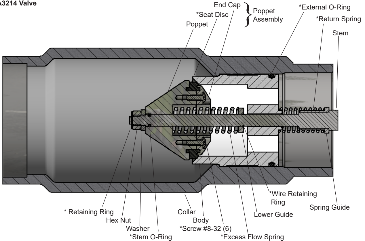
Figure 2 - A3214 Valve
